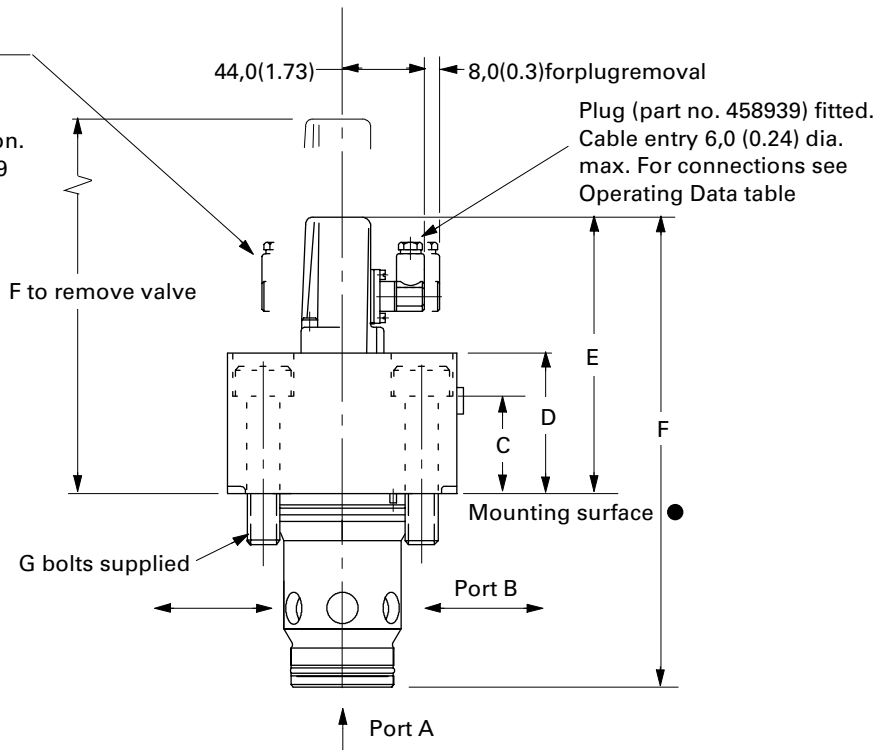
View showing orientation of switch and plug on CVU-25/32/40-SWD models
