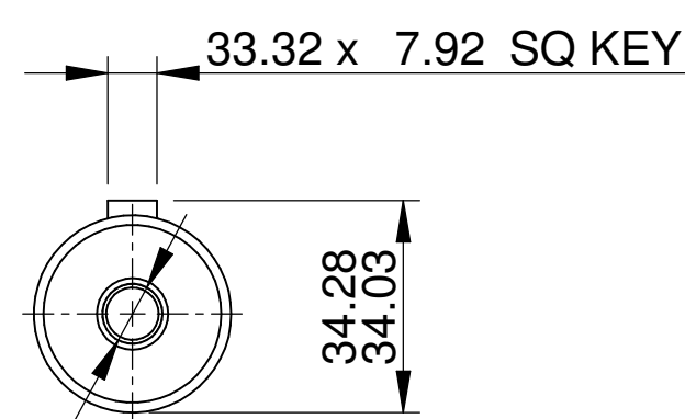
SHAFT DETAILS SCALE 1:1
