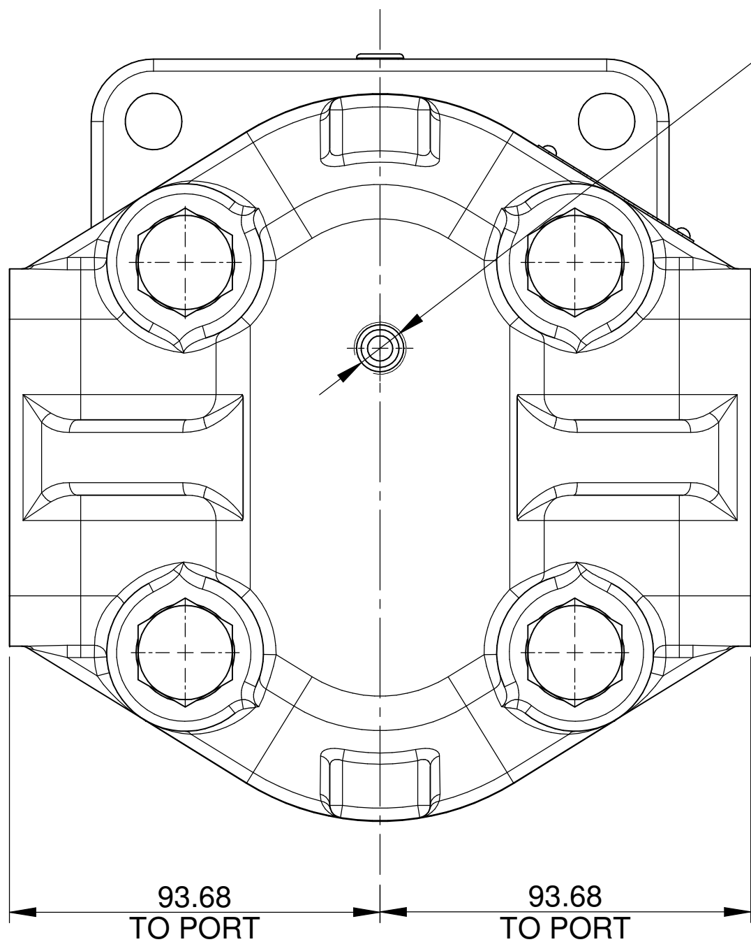
VIEW Z
