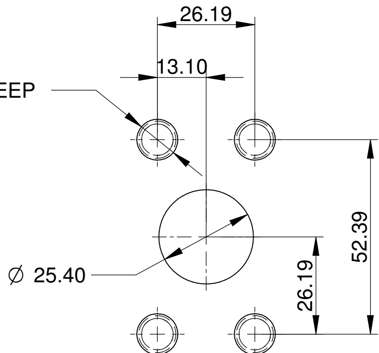
PORT 1" SAE SPLIT FLANGE WITH METRIC THREAD DETAIL 'A' SCALE 1:1
