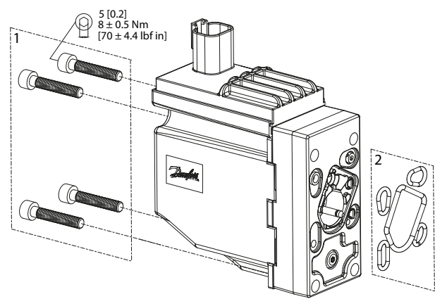
PVEM exploded view
