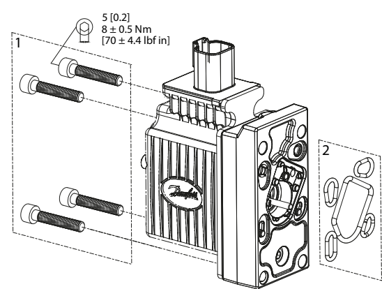
PVEM exploded view
