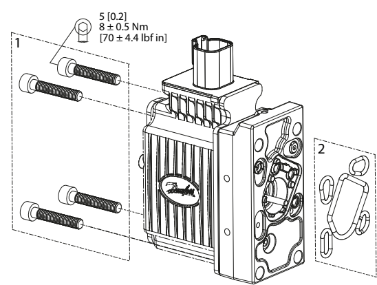
PVEH exploded view
