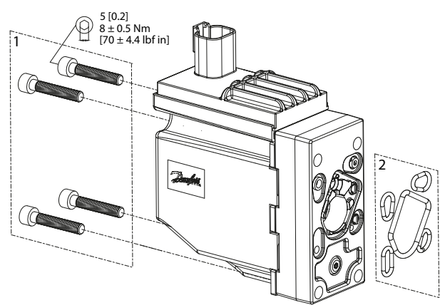
PVEO exploded view
