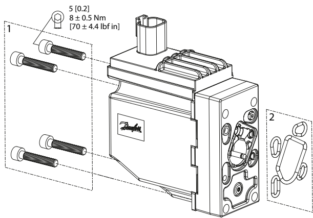
PVEU exploded view
