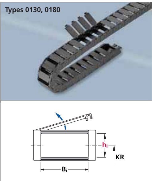
Types 0130, 0180 Cable carriers with hinged, openable brackets
