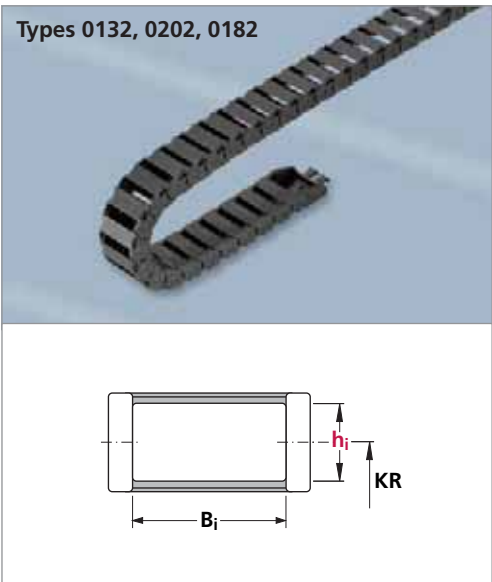
Types 0132, 0202, 0182 Cable carriers with fixed brackets
