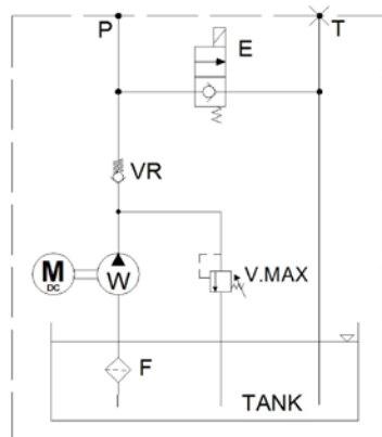
HYDRAULIC CIRCUIT
