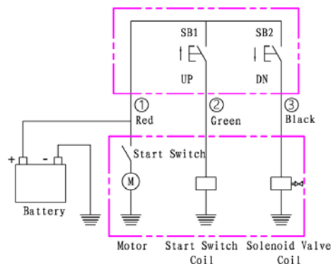
ELECTRICAL CIRCUIT
