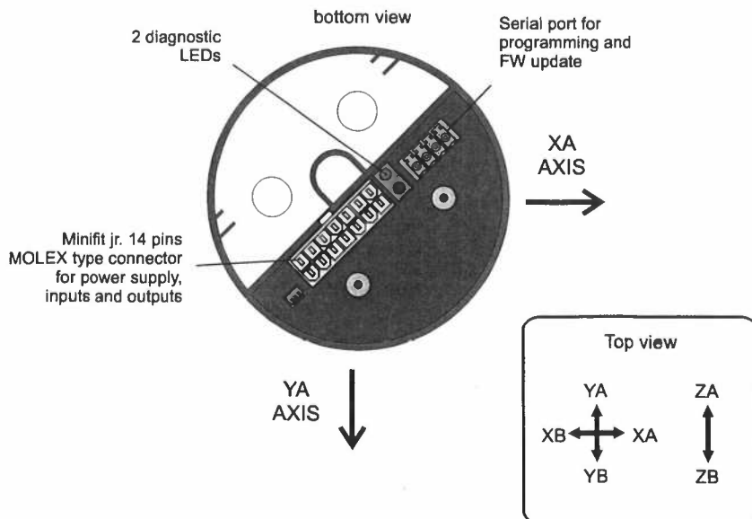
Dual axis joystick (type 115)
