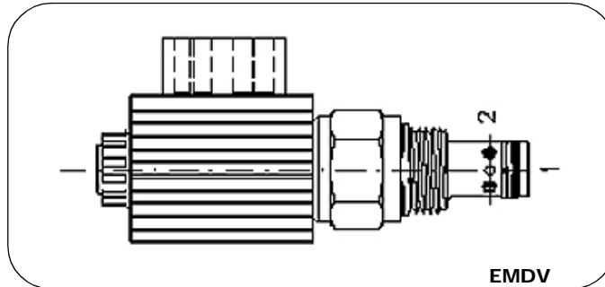
2 way, 2 position, single coil.
