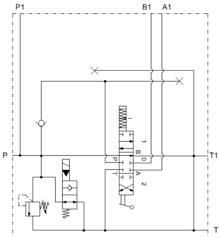
Circuito con UNL – Circuit with UNL (ML1 010A)
