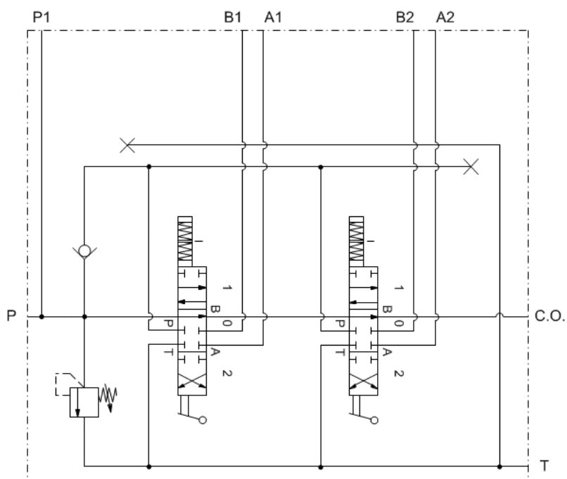
Circuito con Carry over – Circuit with Carry over (ML2 010A 010A)
