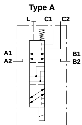
2 positions with ports connected in transit position
