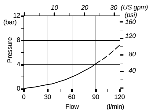
Pressure drop versus flow P \rightarrow A(B)
