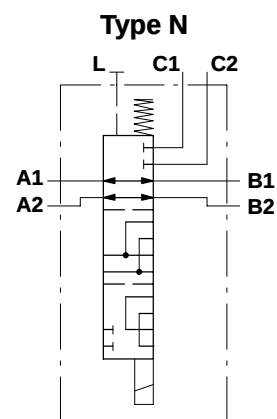
As type A, for right inlet
