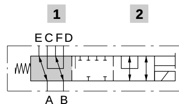
Spool type H
