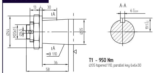
BMS Shaft T1
