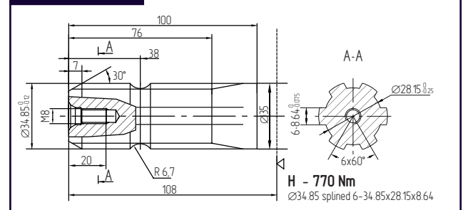
BMS Shaft H
