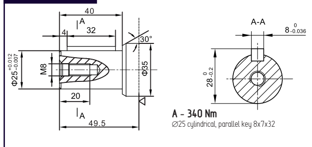
BMS Shaft A
