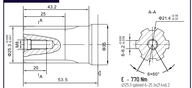
BMS Shaft E
