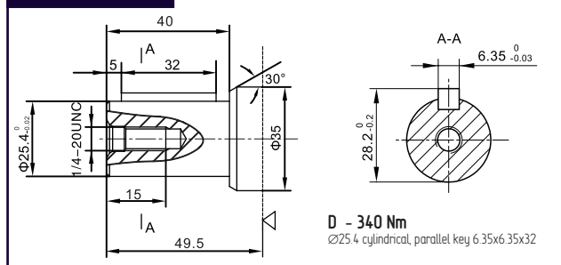
BMS Shaft D
