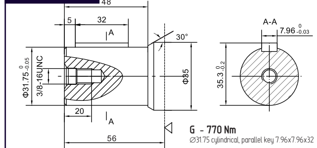
BMS Shaft G
