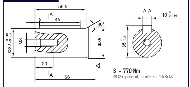
BMS Shaft B
