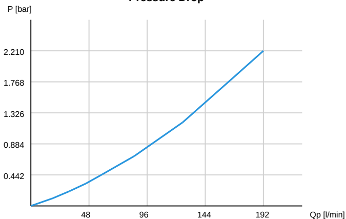
Pressure Drop
