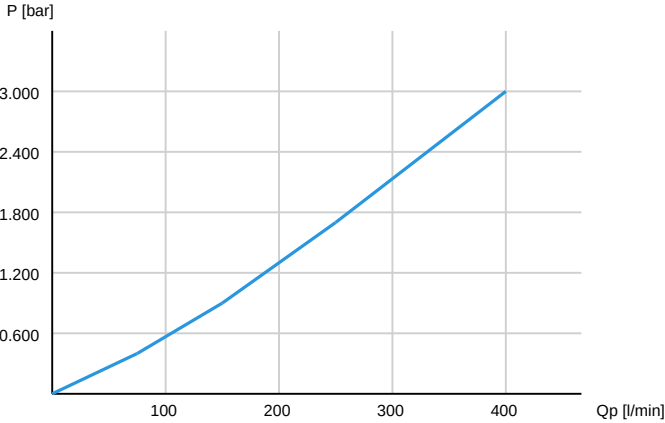
Pressure Drop
