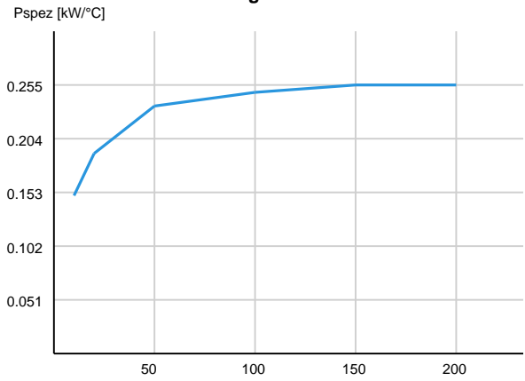
Cooling Performance*
