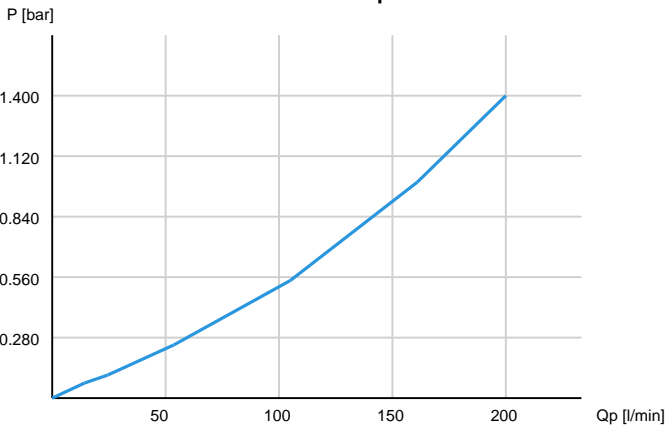
Pressure Drop
