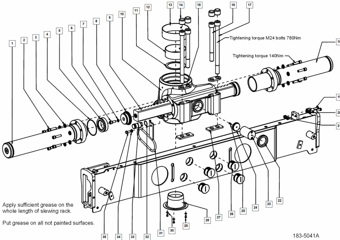
1835041 - Slewing group assembly (s/n 055 0932 and up)
