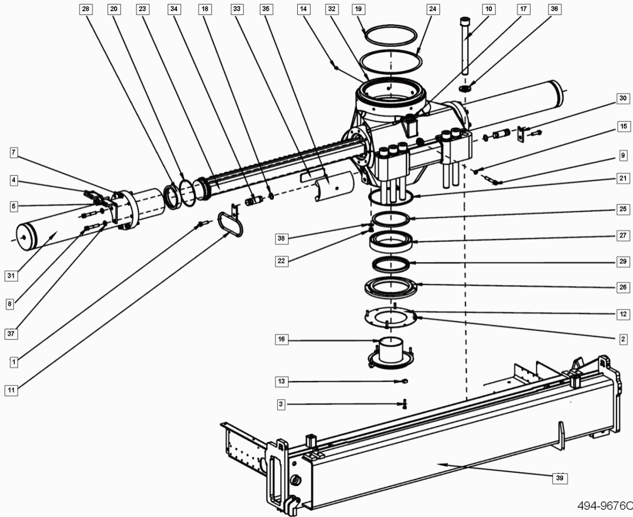
4949676 - Assembly parts base
