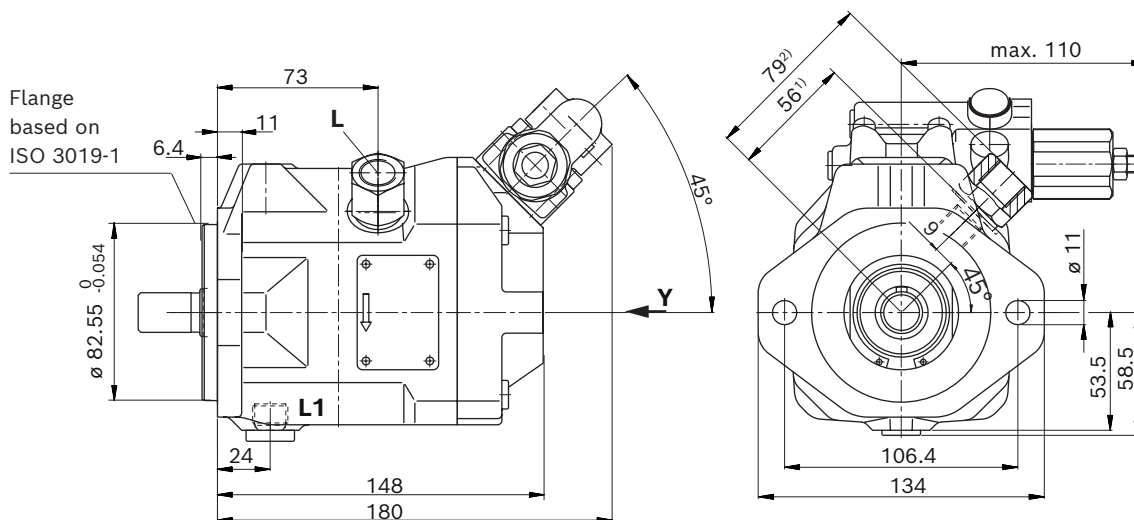
▼ View Y Valve mounting for clockwise rotation
