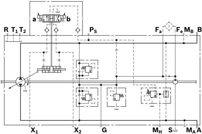
▼ Circuit diagram size 63
