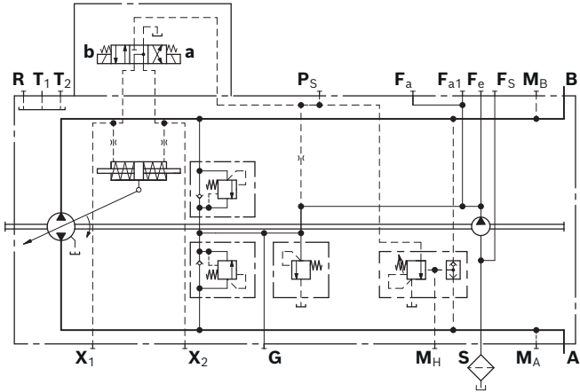
▼ Circuit diagram, standard version 1)
