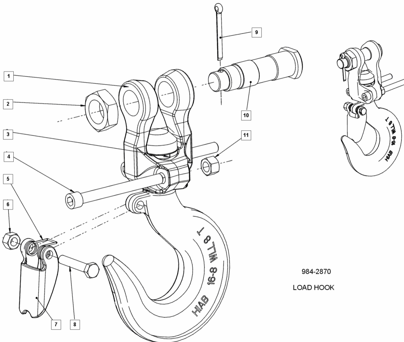
9842870 - Load hook
