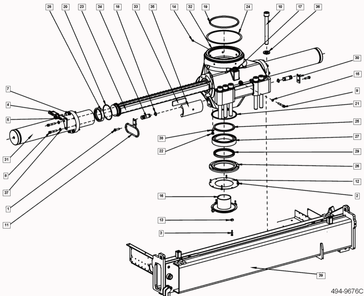
4949676 - Assembly parts base
