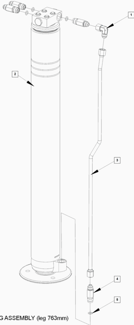
6001274 - Stabilizer leg assembly
