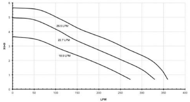
9303C-HM5C-SP & 9303S-HM5C METRIC-SP
