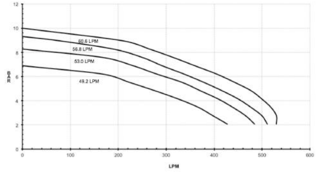
9303C-HM5C & 9303S-HM5C METRIC 9303C-HM5C-U & 9303S-HM5C-U
