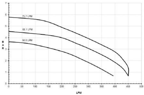
9303C-HM4C-SP & 9303S-HM4C-SP METRIC
