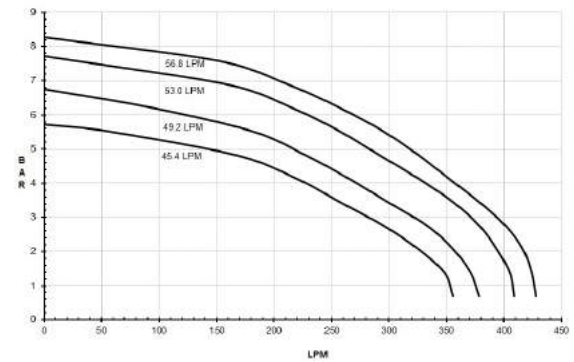
9303P-HM5C & 9303P-HM5C METRIC
