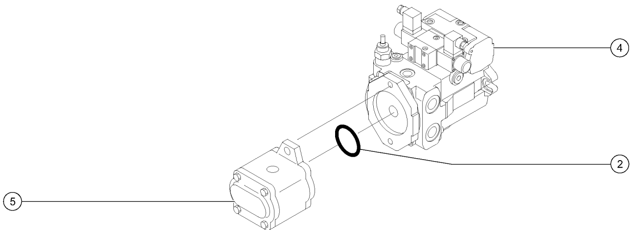
Hydraulic Pump Assembly - Non-oscillating Models
