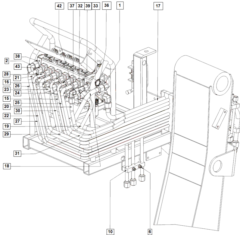
4961196 - Pipe kit high seat V91/V91M
