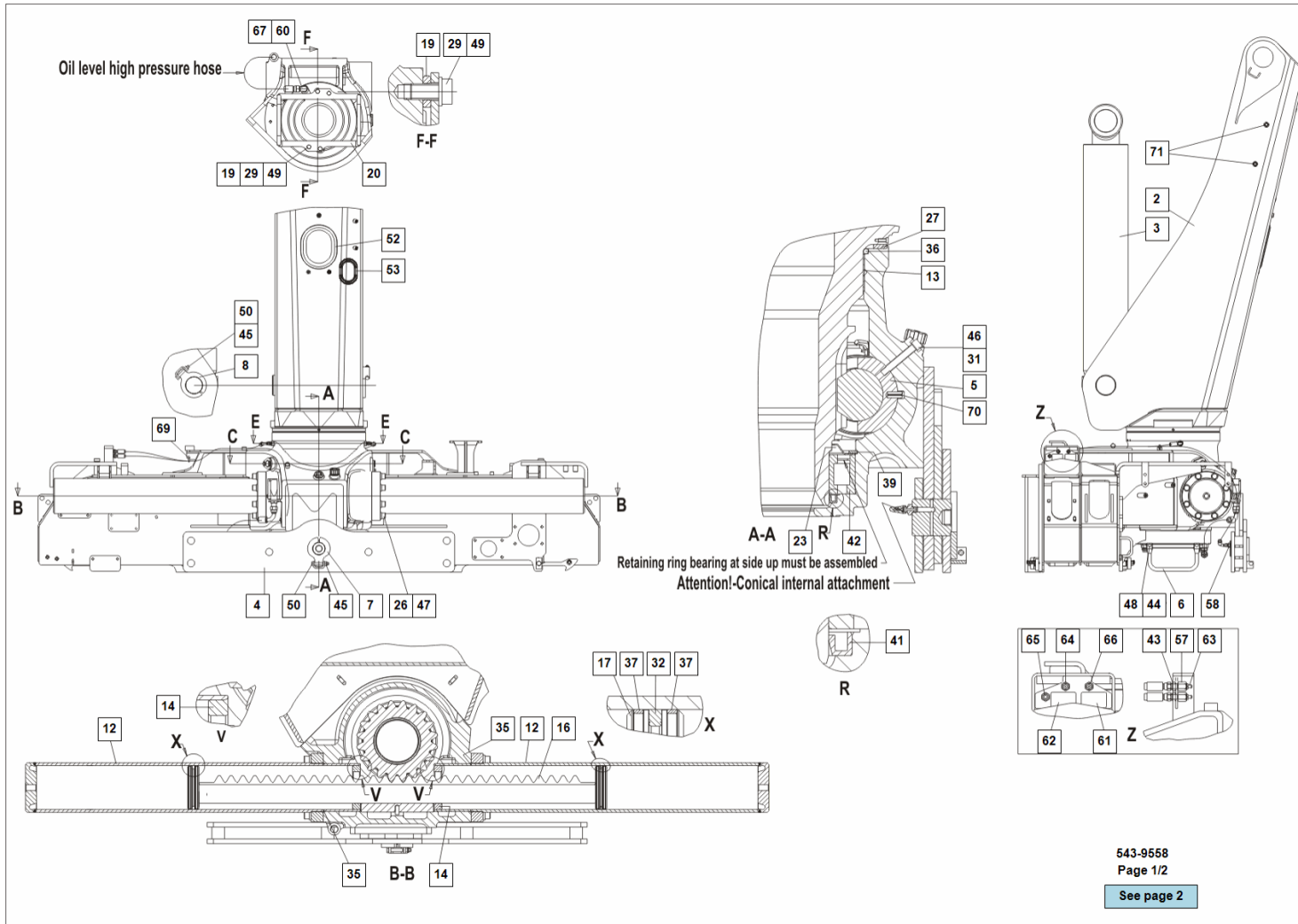
5439558 - Base mounting (founded base) (Page 1/2) (3350270 and from 3350316, except 322,323,326,327)
