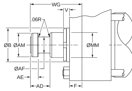
6.00" Bore
