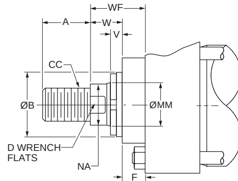
8.00" Bore
