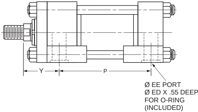
Dimensions — Manifold Ports for Single and Double Rod Cylinders
