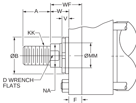
6.00" Bore
