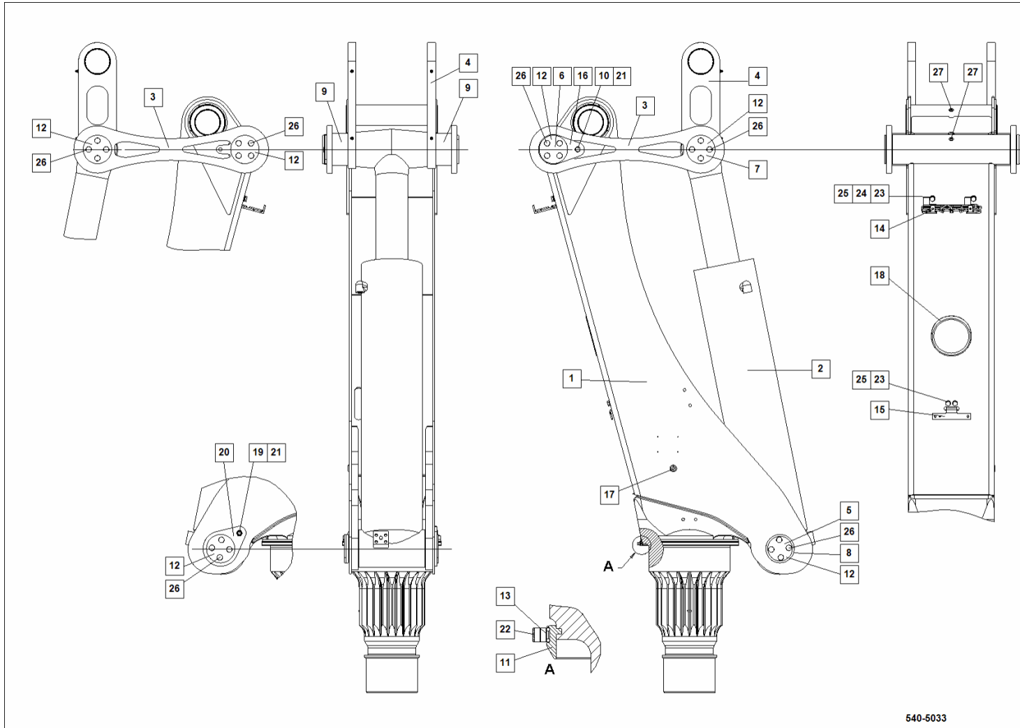
5405033 - Loader body- cylinder
