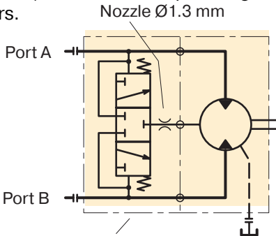
Hydraulic schematic.
