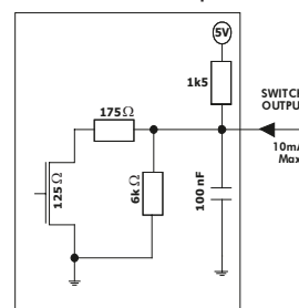
Equivalent circuit for the switch output
