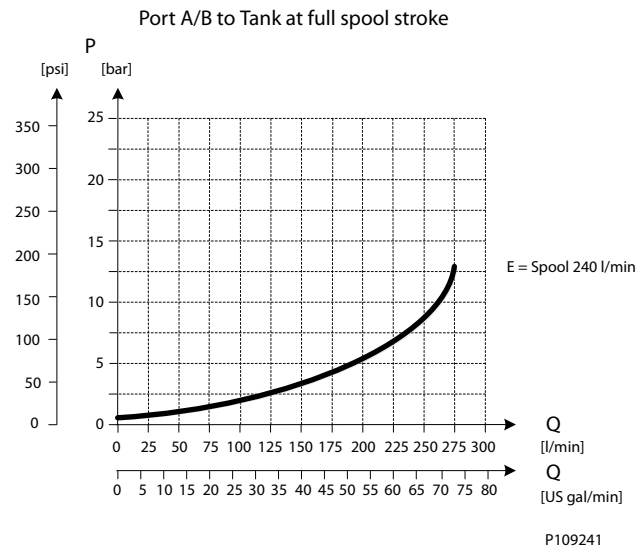
PVB 128 Downstream Performance
