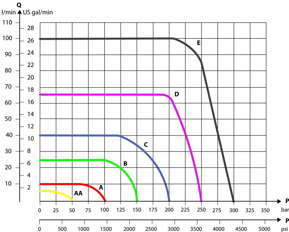
PVB pressure compensated for LS A/B characteristics
