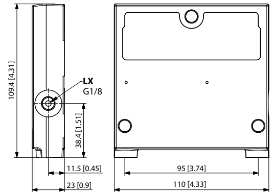
PVSI with LX-connection dimensions
