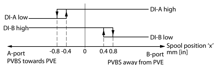
Direction indication feedback
