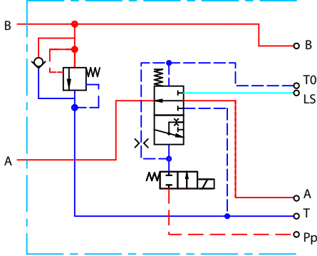
Multi-valve schematic
