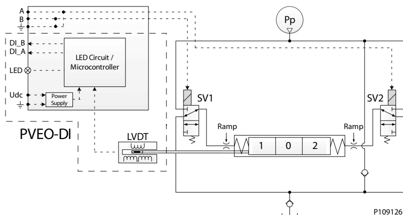
PVEA-DI functionality
