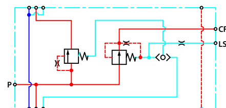
Open Center PVSPM giving priority to OSP+PVB
