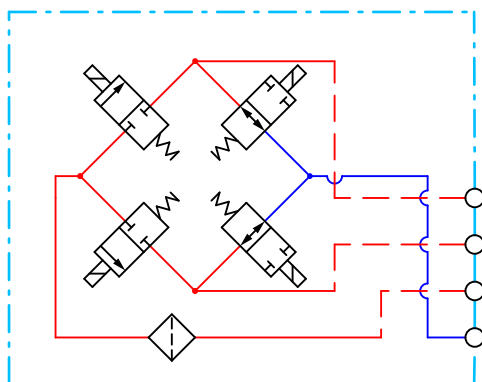
PVEP schematic
