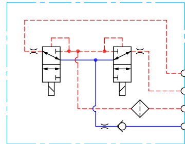
PVEO-R schematic
