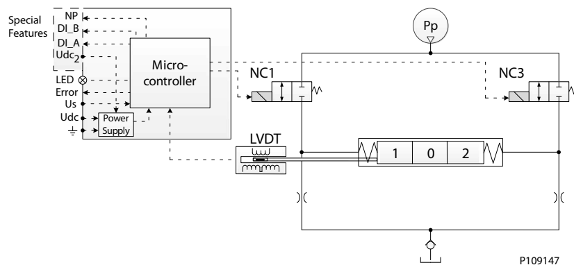
PVEH functionality
