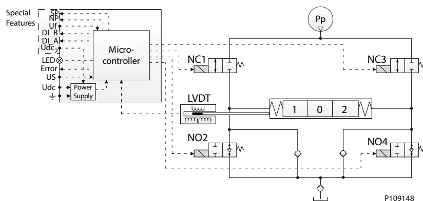
PVEH functionality
