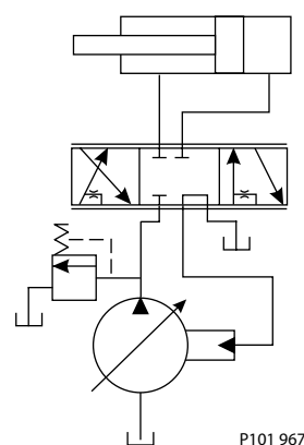
Load sensing circuit
