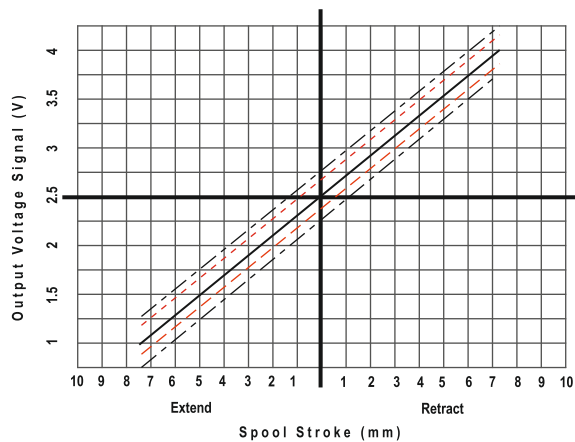
Spool Position Sensor Output Signal for 120EHP5482
