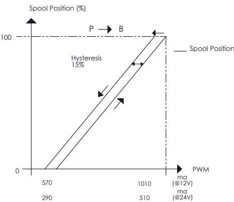
Hysteresis
