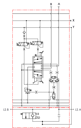
Normally Closed LSB Active
