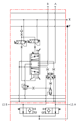
Normally Open LSA+LSB Active
