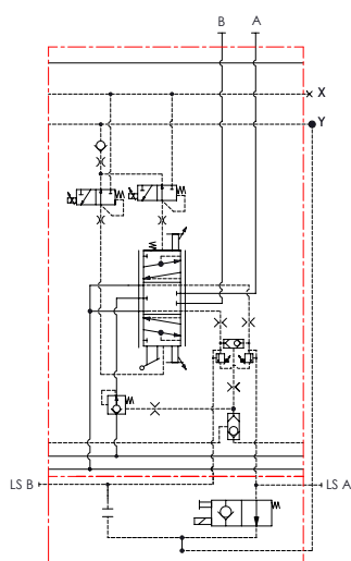
Normally Open LSA Active
