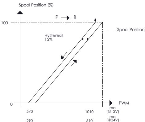
Hysteresis
