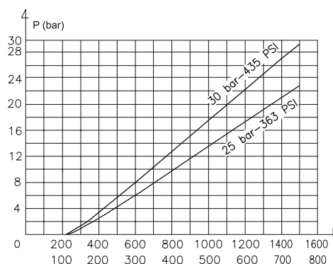
Reduced pressure (bar) vs. Current (mA) 12 V and 24 V Coil
