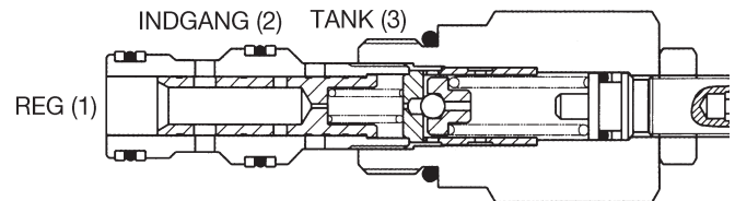
Overcenterventil
