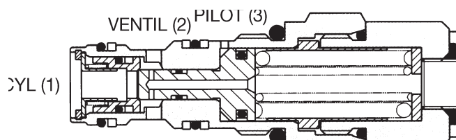
Overcenterventil
